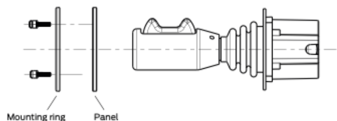
Mounting arrangement
